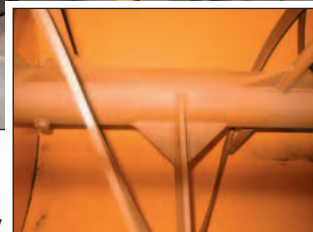
Double, counter-rotating screw
