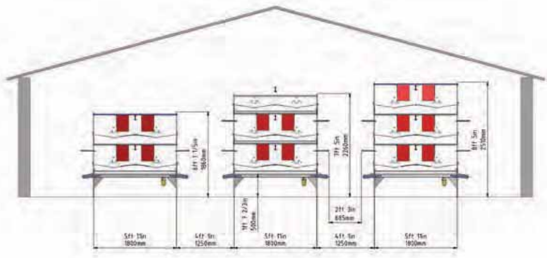
Example of two and three tier nest layout
